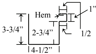
Box Gutter without Leg
